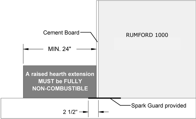
FIGURE 11 RAISED HEARTH EXTENSION
