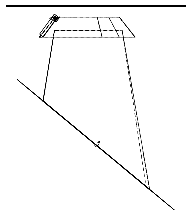
FIGURE 13 STORM COLLAR POSITION
