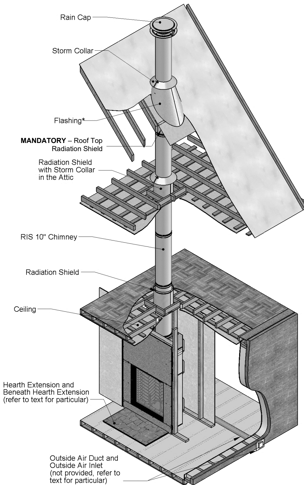
FIGURE 1 GENERAL INSTALLATION OVERVIEW
