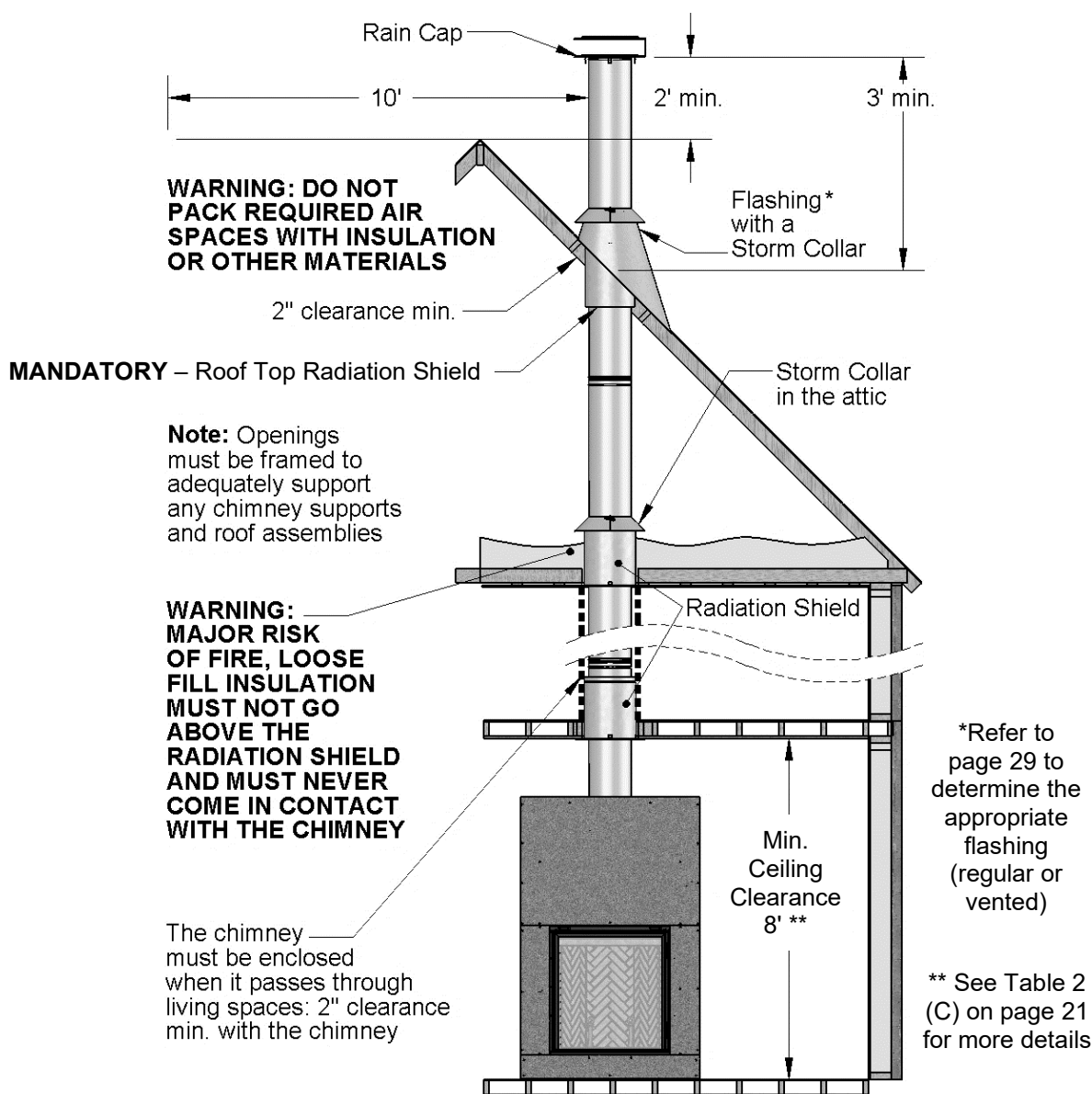
FIGURE 4 GENERAL CHIMNEY REQUIREMENTS
