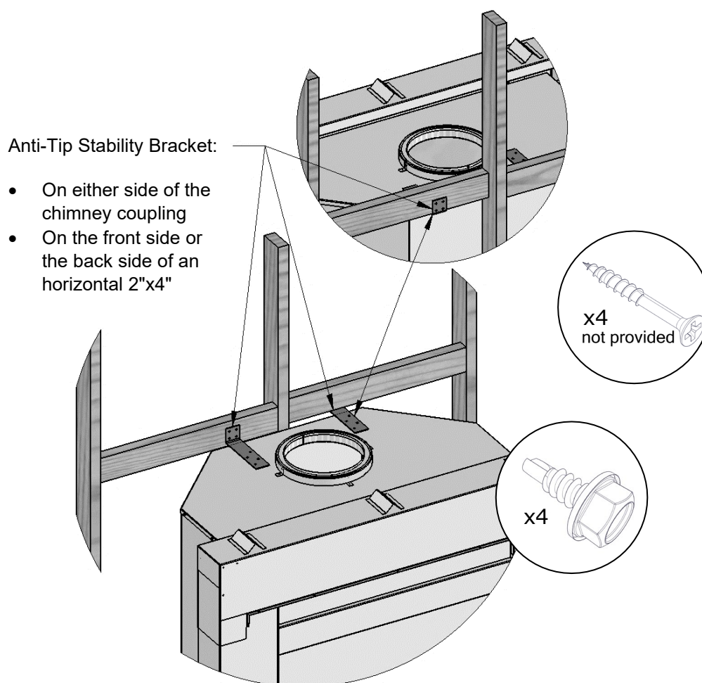
FIGURE 7 ANTI-TIP BRACKET INSTALLATION
