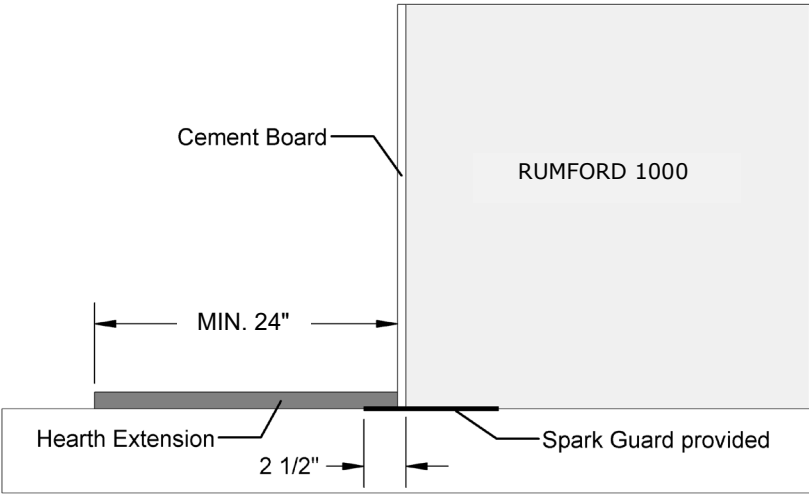
FIGURE 9 STANDARD HEARTH EXTENSION
