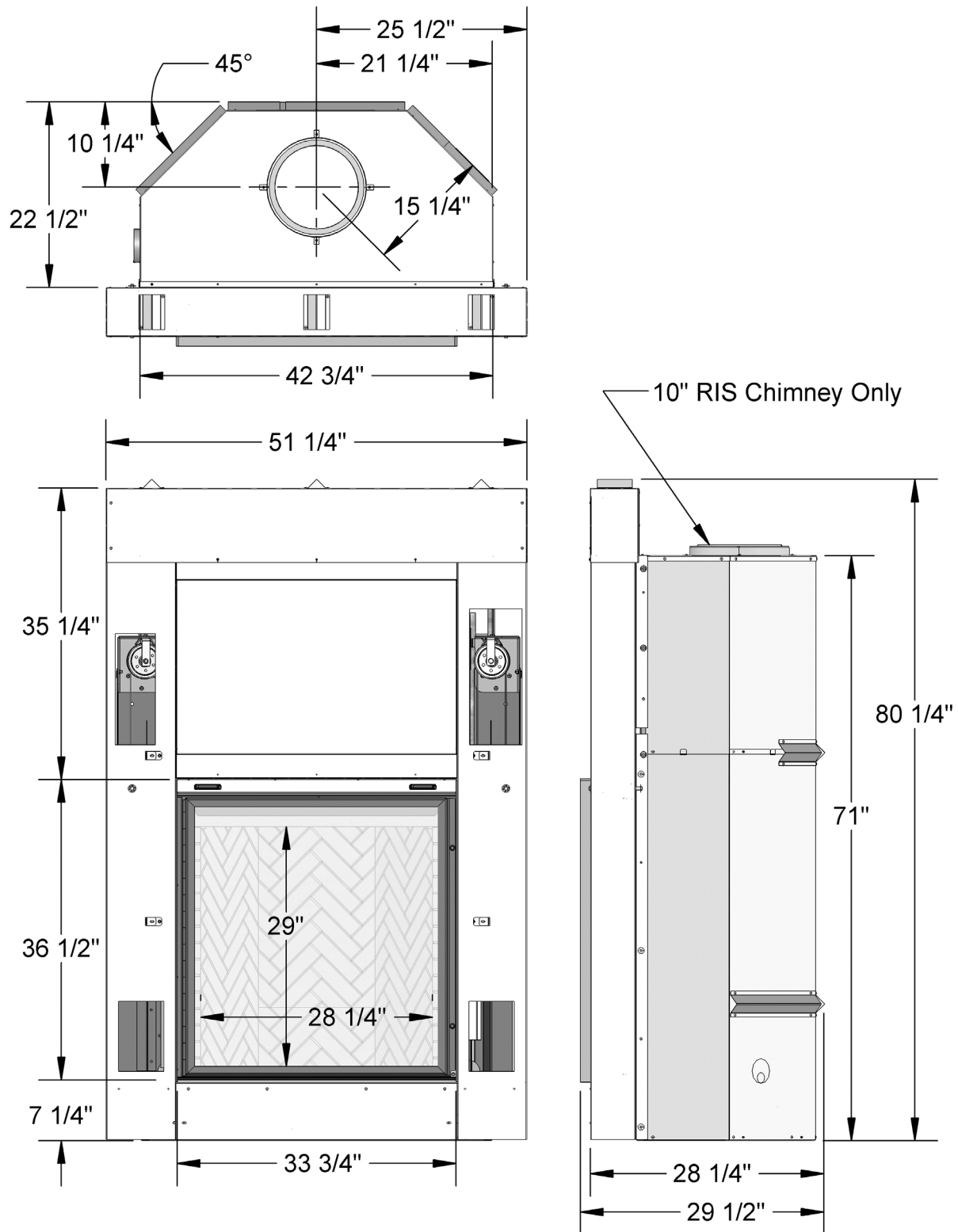
FIGURE 2 FIREPLACE DIMENSIONS
