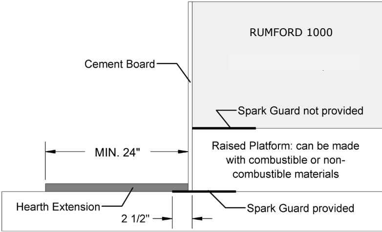
FIGURE 10 RAISED FIREPLACE
