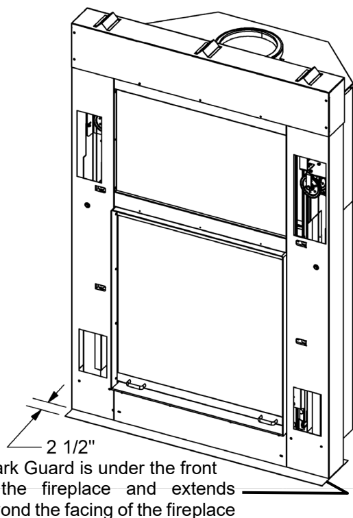
FIGURE 6 SPARK GUARD INSTALLATION
