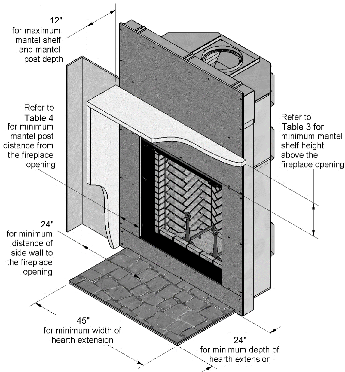
FIGURE 8 FIREPLACE CLEARANCES (SEE TABLE 2)
